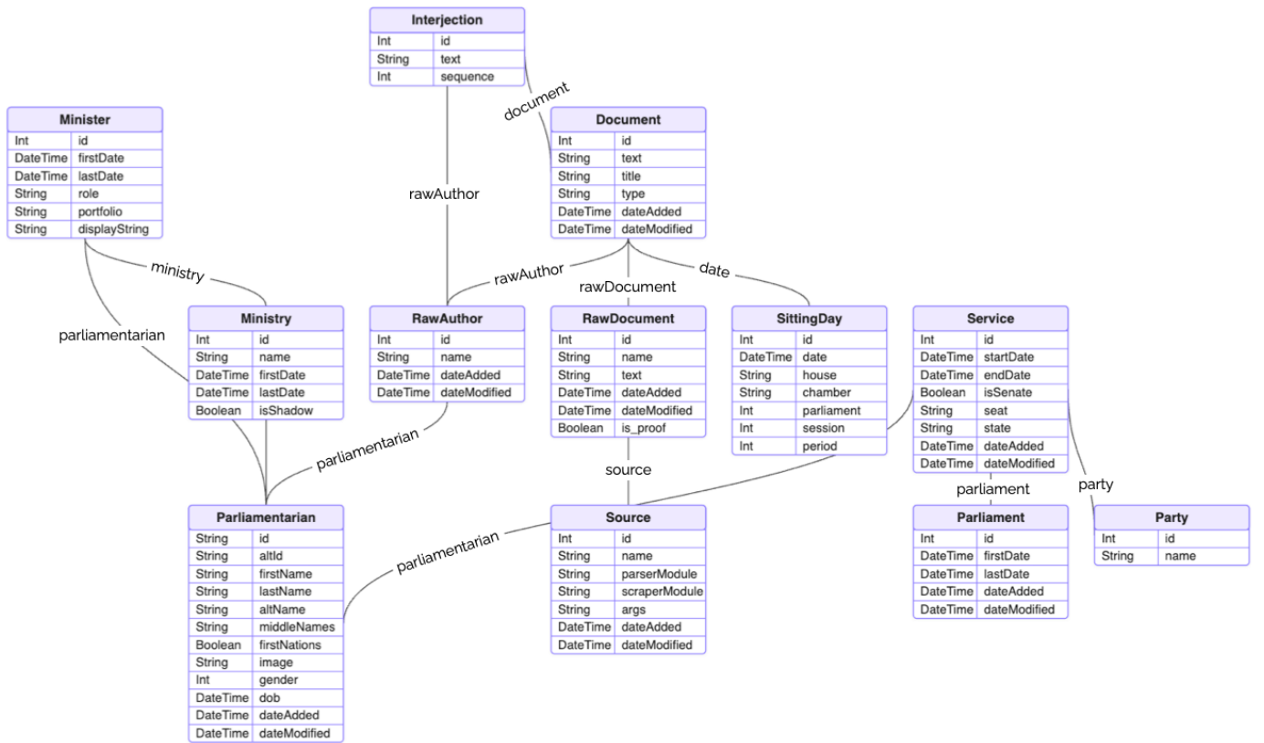
Figure 7: Entity–relationship diagram of the Hansard relational database. Core parliamentary contributions ( Document , Interjection ) are linked to sitting-day provenance ( SittingDay , Source , RawDocument ) and to speaker metadata ( Parliamentarian , Service , Party , Minister , Ministry ) via persistent Parliamentary Handbook identifiers. Self-referential Document relationships capture question–answer pairings.
